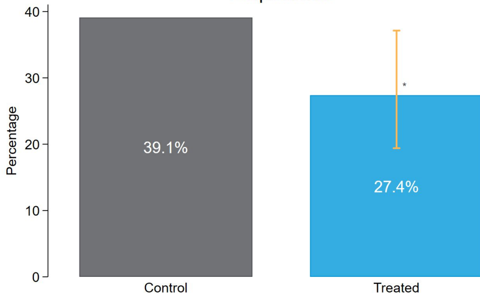
Dropout rate
