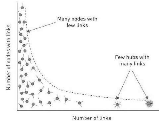
d) Scale-free
