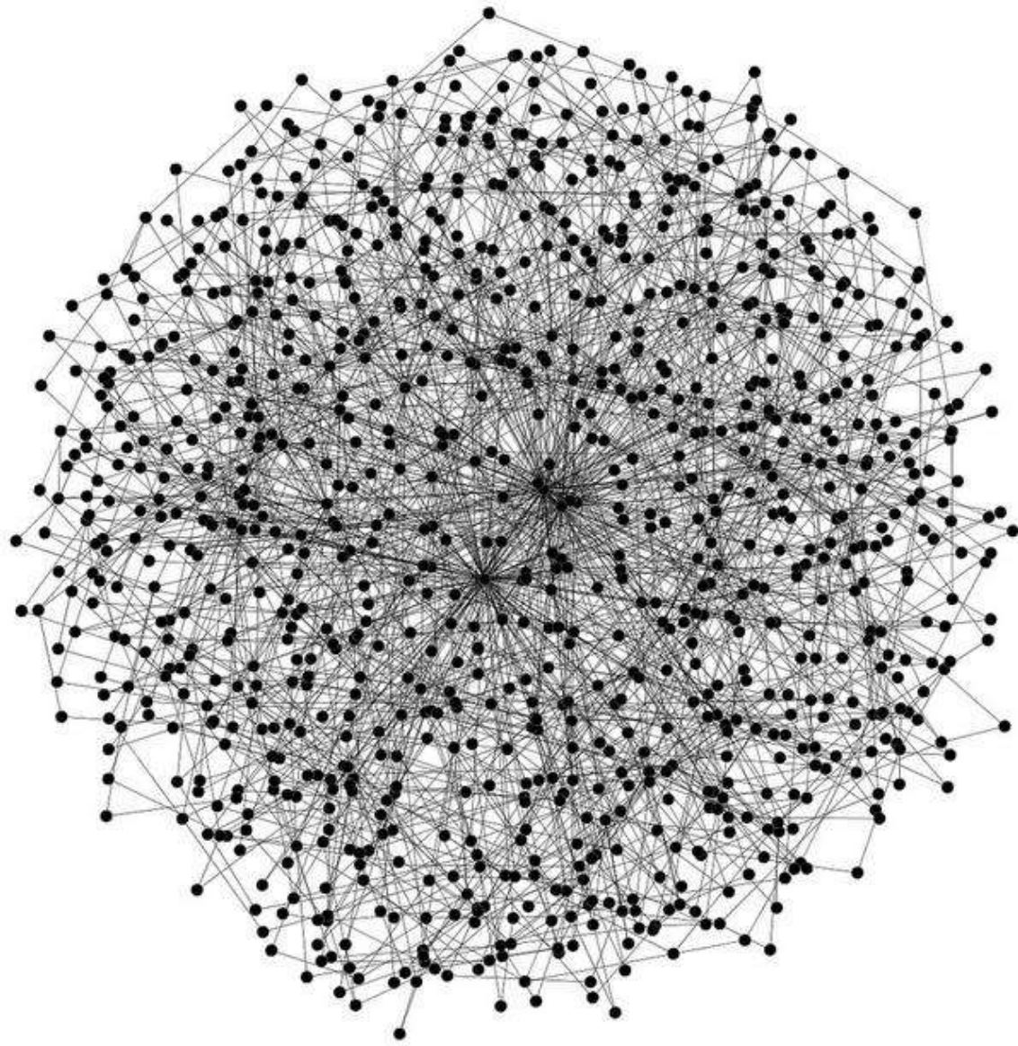
Red aleatoria
